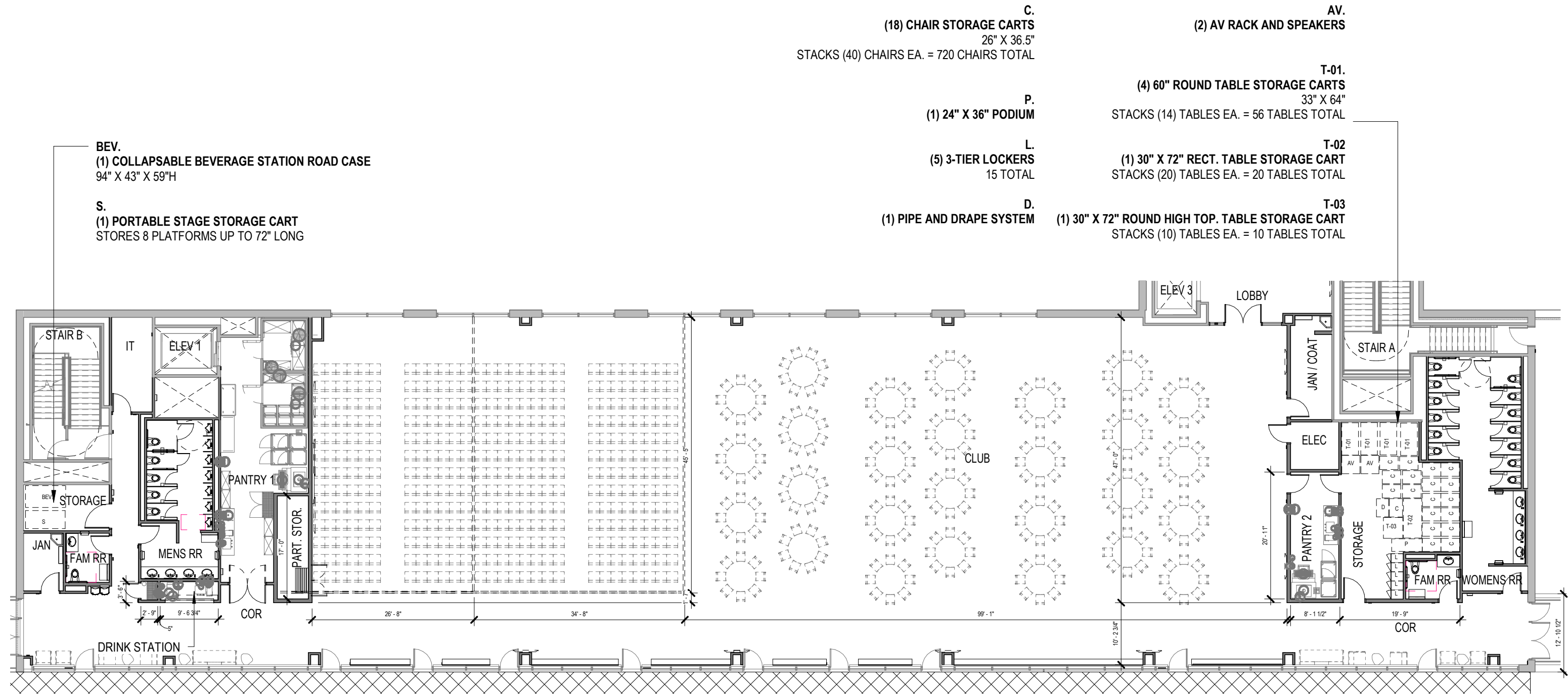
1 LEVEL 04 - CLUB LAYOUT - BANQUET AND SPEAKER 1/16" = 1'-0"
